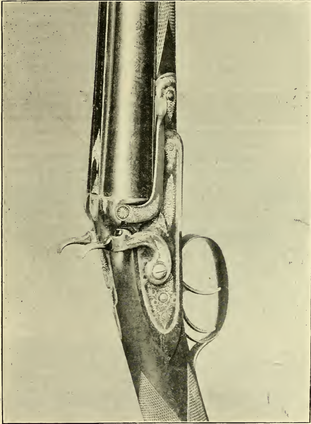
[Needham's Snap-action Mechanism.
